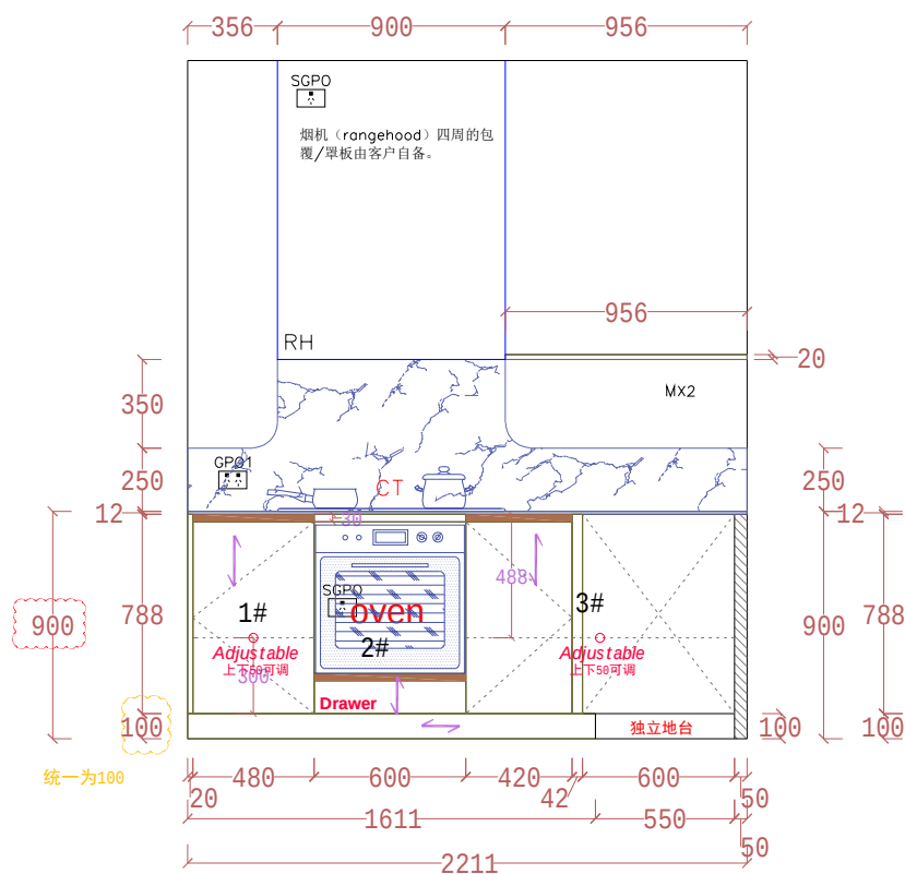
ELEVATION C KITCHEN
