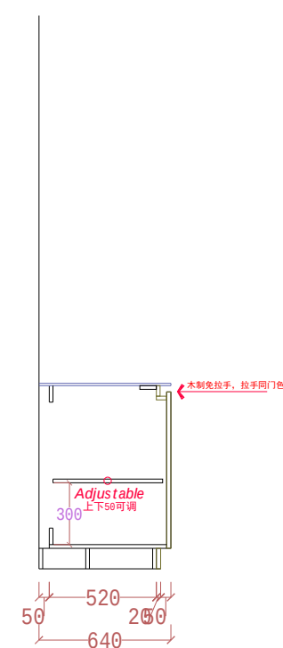
SECTION VIEW 3
