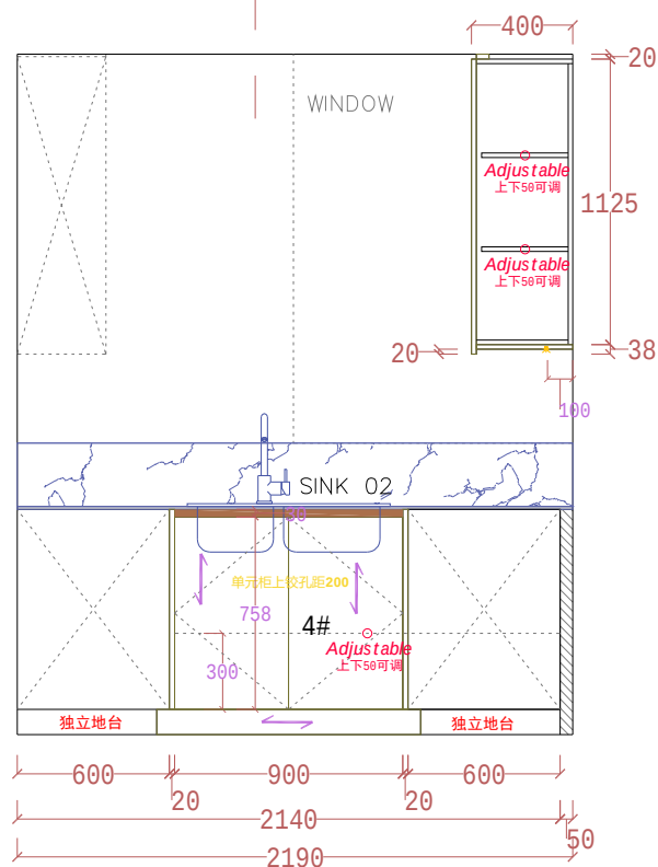
ELEVATION D KITCHEN
